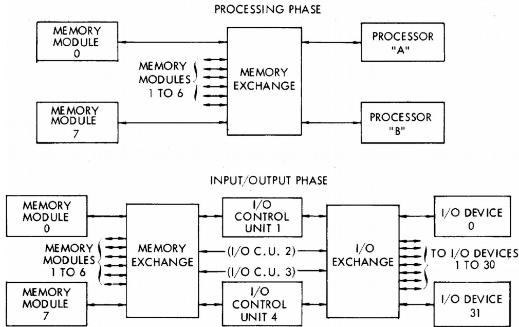
Illustration 2: Basic machine overview
